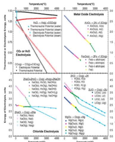
Calculated potential to electrolyze selected oxides (top) and chlorides (bottom). The indicated decrease in electrolysis energy, with increase in temperature, provides energy savings in the STEP process in which high temperature is provided by excess solar heat. Licht, 2009. Click to enlarge.
