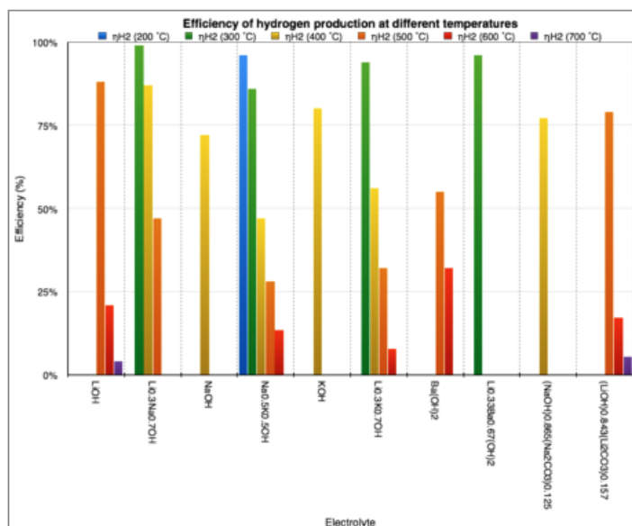
Measured coulombic efficiency of hydrogen generation ( \eta_{H_2} ) in various molten hydroxide electrolytes at various temperatures. Data source: Li et al. Click to enlarge.
