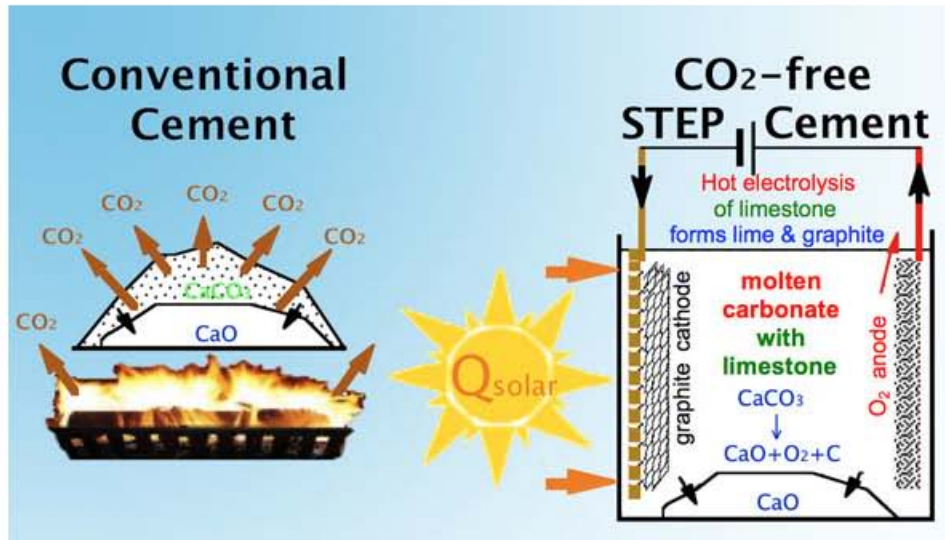
Conventional thermal decomposition production of lime (left) versus STEP direct solar conversion of calcium carbonate to calcium oxide (right) eliminating CO 2 . (Image: Dr. Licht, University of Washington)
