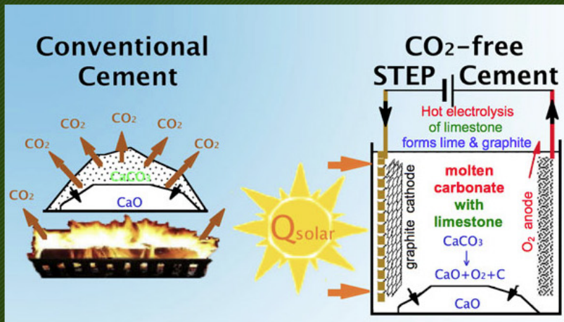
Conventional thermal decomposition production of lime (left) versus STEP direct solar conversion of calcium carbonate to calcium oxide (right) eliminating CO 2 . (Photo source: Dr. Licht, University of Washington)
