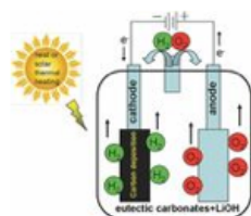
One-pot electrolytic process produces H 2 and solid carbon from water and CO 2 . Li et al. Click to enlarge.
