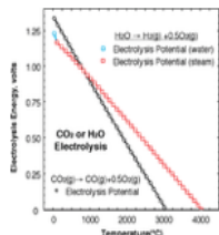
Calculated potential needed to electrolyze carbon dioxide or water. The indicated decrease in electrolysis energy, with increase in temperature, provides energy savings in the STEP process. High temperature is accessible through excess solar heat. Licht, 2009.
